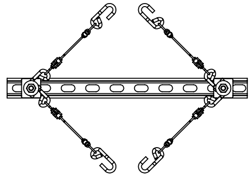
OVERHEAD VIEW ALTERNATE SPLOYED CABLE BRACE PATTERN
